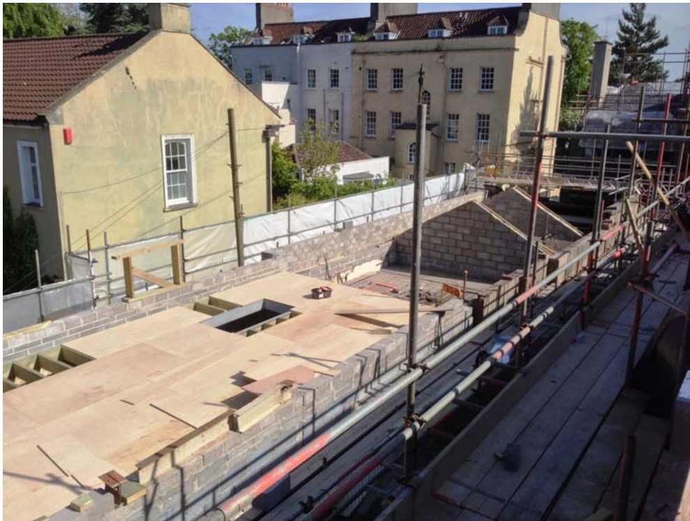
The above photograph shows the works progress on the former stable block.
